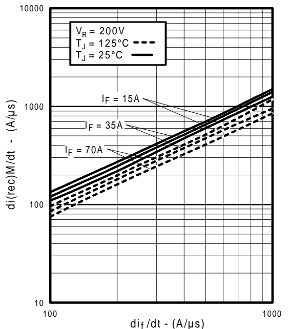
Fig. 8 - Typical di(\text{rec})M/dt vs. di/dt , (per Leg)
