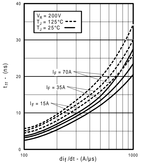
Fig. 6 - Typical Recovery Current vs. di/dt , (per Leg)
